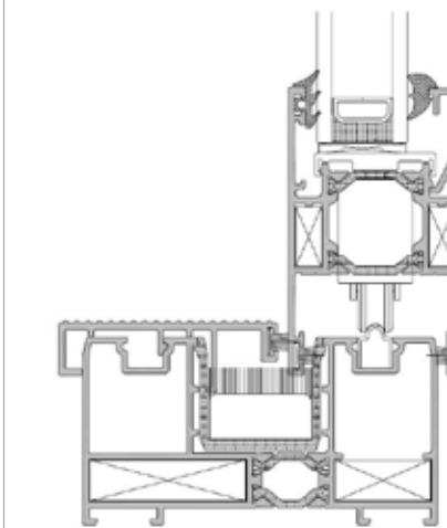
Cill detail
